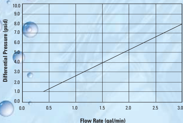
Degas Module Flow Rate vs. Pressure
