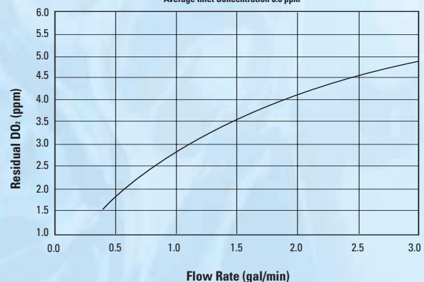
Degas Module Flow Rate vs. Residual DO 2 Average Inlet Concentration 8.0 ppm
